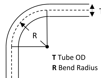
Figure 1 Recommended Bend Radius
