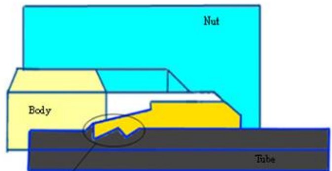
Metal Sleeve cutting into tube
