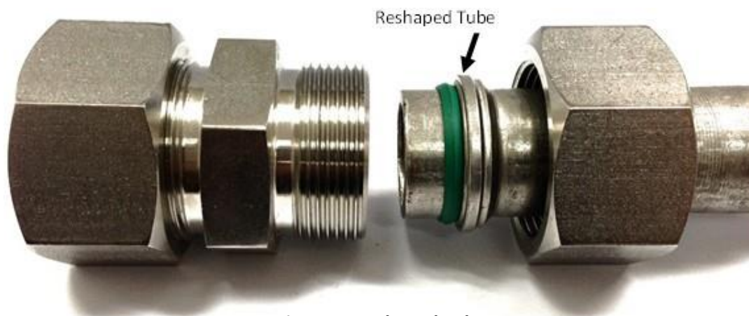
Figure 3: Reshaped Tube
